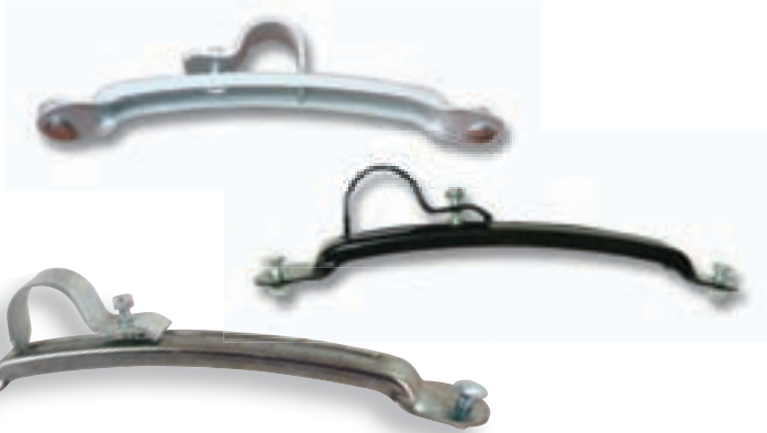
ÇAMURLUK BORUSU, 3 DELİK, Ø42 TRAILER MUDGUARD TUBE, 3 HOLE, Ø42 4-TR405701 KISA TİP, 57cm / SHORT TYPE, 57cm 4-TR408001 UZUN TİP, 80cm / LONG TYPE, 80cm
