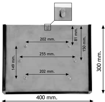
Cod. 91297 Portapanello inox con gancio e bordo per cartelli 400x300 mm. Stainless steel panel holder with safety hook and black PVC coated edge for panels 400x300 mm.
