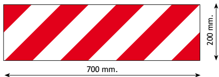
Cod. 80961 Kit pannello alluminio trasporto eccezionale 700x200x2 mm. Kit aluminium panel white reflecting and red fluorescent. 700x200x2 mm.
